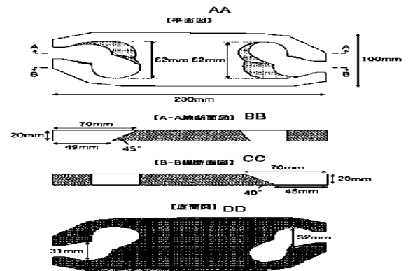
AA Planar diagram BB A-A cross-sectional diagram CC B-B cross-sectional diagram DD Bottom diagram
