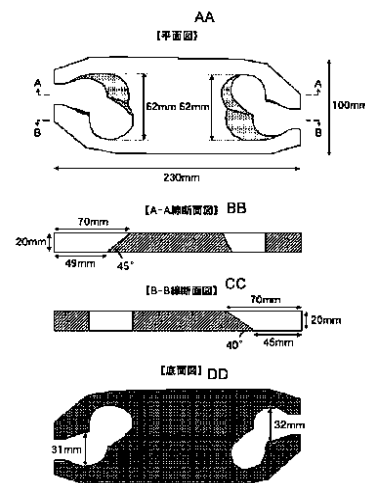
AA Planar diagram BB A-A cross-sectional diagram CC B-B cross-sectional diagram DD Bottom diagram
